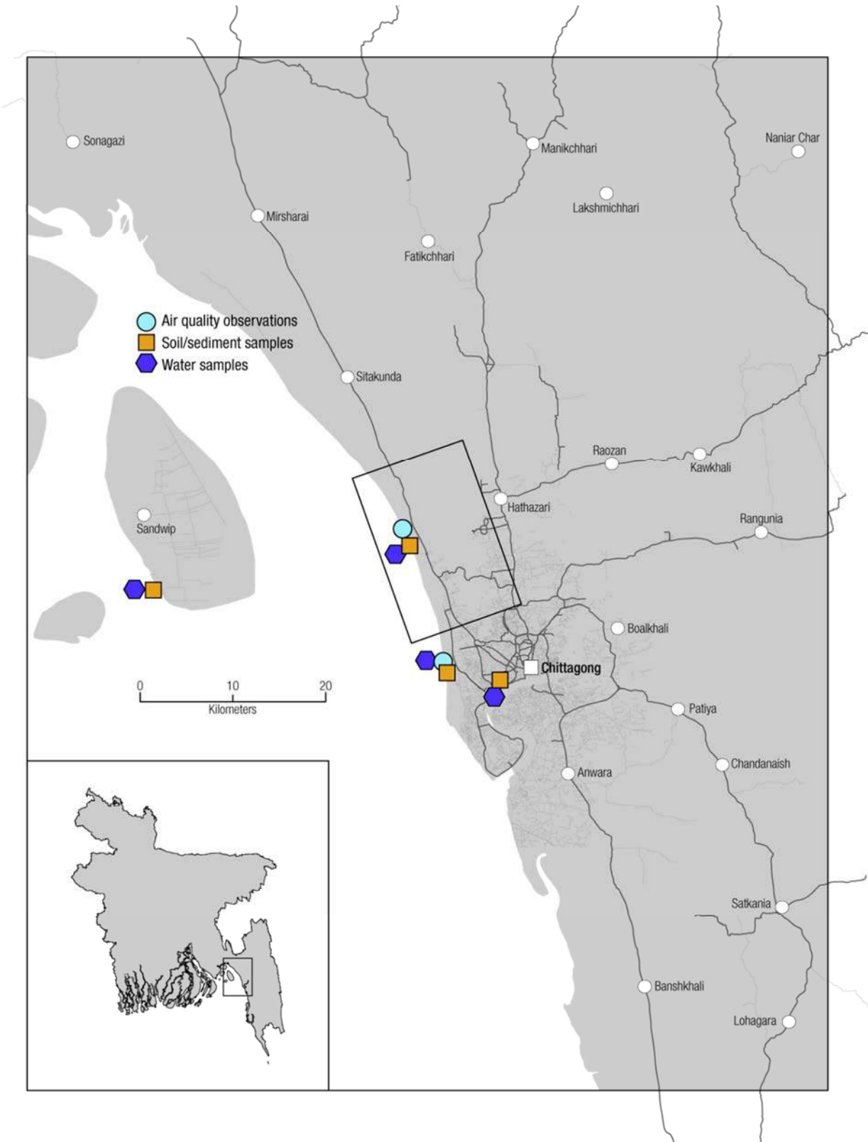
Figure 3.12 Location of air, water and sediment sample collection/observation points in the coastal environment of Chittagong, Bangladesh
