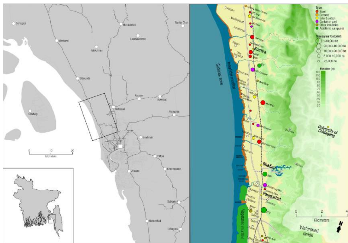
Figure 1.1 Map showing the coastal zone of Chittagong and enlarged is the ship recycling area at Sitakunda coast
