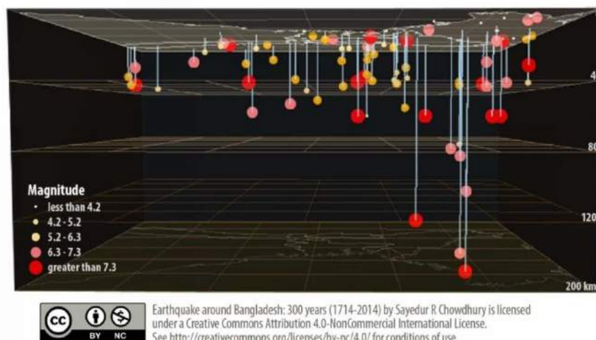
Figure4.7 Earthquake around Bangladesh (source: mapsnmaps.blogspot.com2014)
