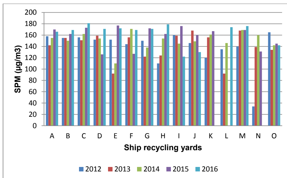
Figure 3.9. Level of suspended particulate matter in ambient air of ship recycling yards at Sitakunda, Chittagong (from DoE)
