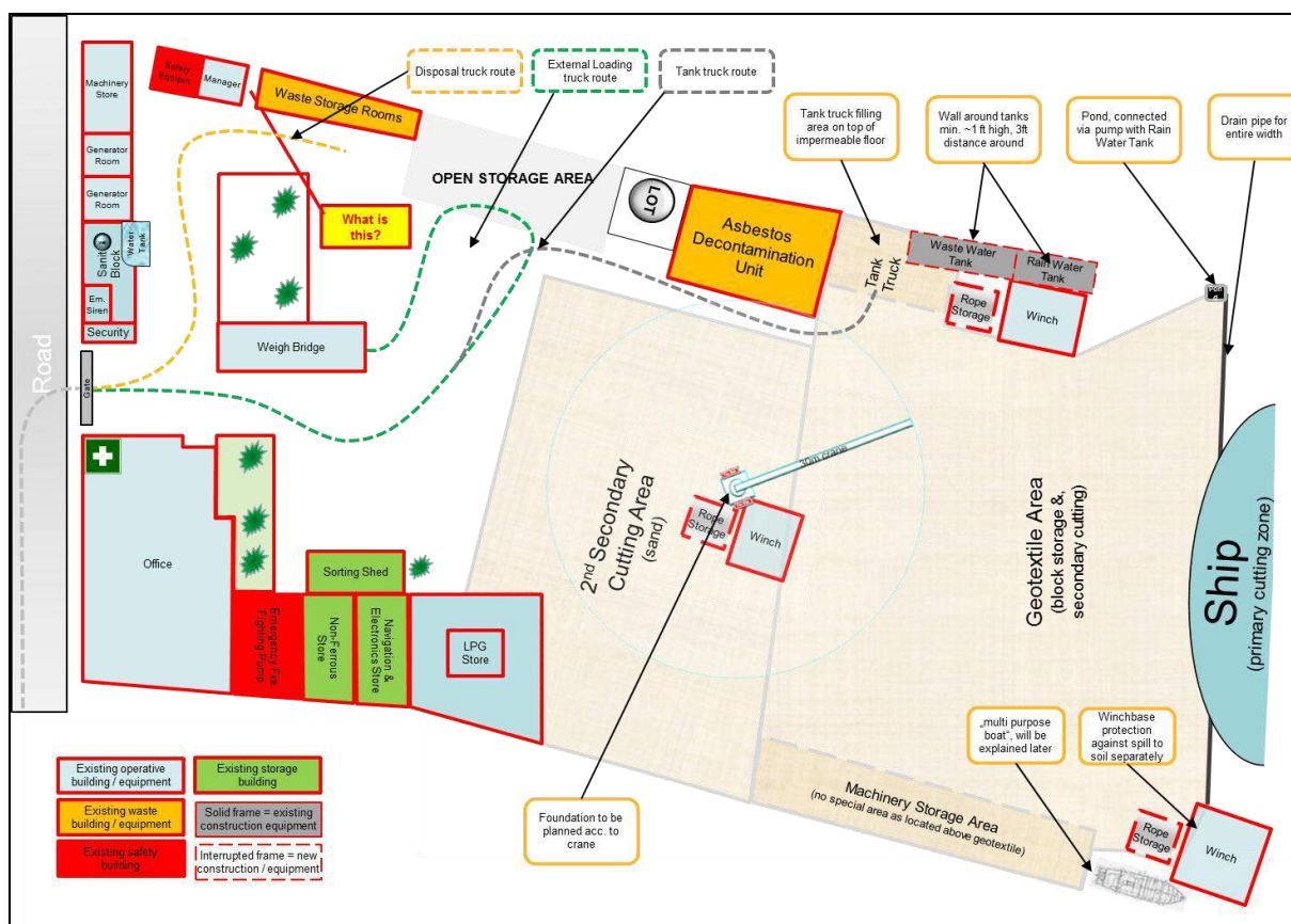
Figure 4: Example layout of SRF in another recycling country
