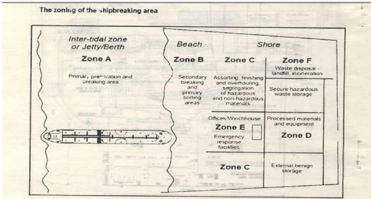
Figure 3: Zoning of the yard, a requirement as part of SRFP (Source: SBRR, 2011)
